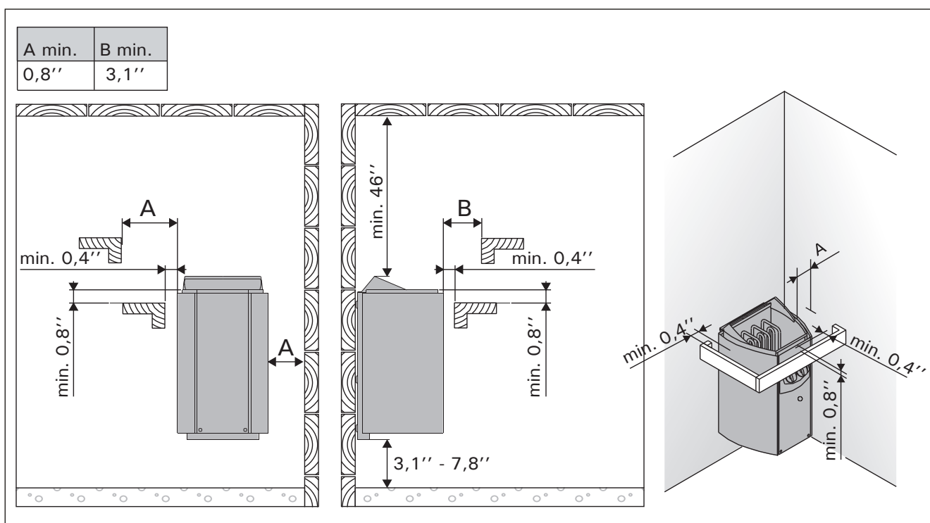
Figure 5. Minimum safety distances
